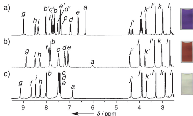
Figure 4. ^1\text{H} NMR spectra (400 MHz, \text{CD}_3\text{CN} , room temperature) and photographs of the solutions of a) complex 2\supset\text{C}_{60} , b) complex 2\supset\text{C}_{70} , and c) 3 formed upon the addition of \text{Hg}(\text{OTf})_2 (2 equiv) to the 2\supset\text{C}_{60} complex.
